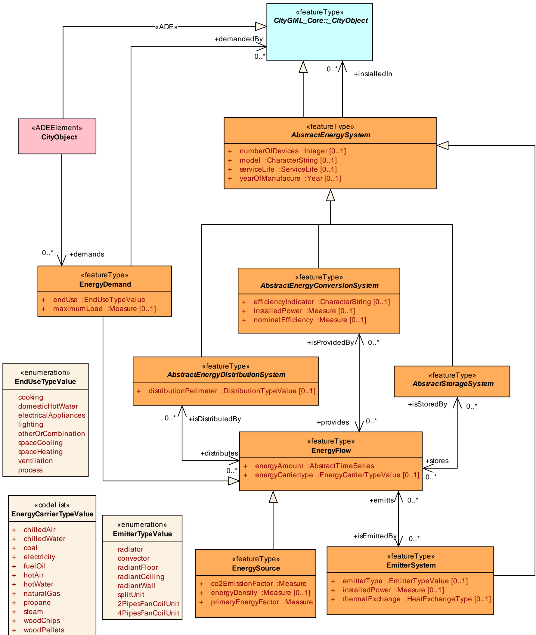
Diagram: EnergySystem-Base classes
